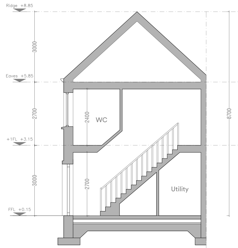
House Type L1 Semi- Detached Section A.A
